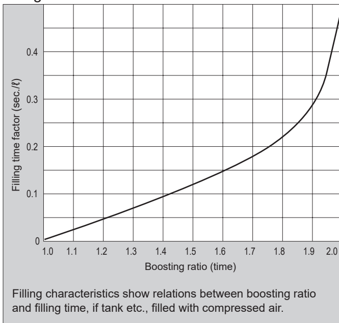
Filling characteristics
